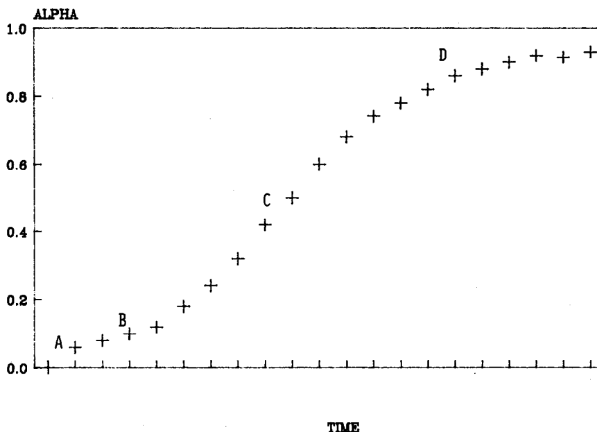
Fig. 1. A typical plot of \alpha vs. time for a solid state reaction.
